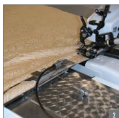
1. 1-Thread blind stitch including puller transport
