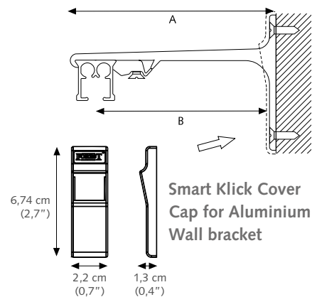
SK Wall bracket aluminium double
