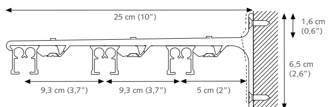
SK Wall bracket aluminium triple 25 cm (10'')
