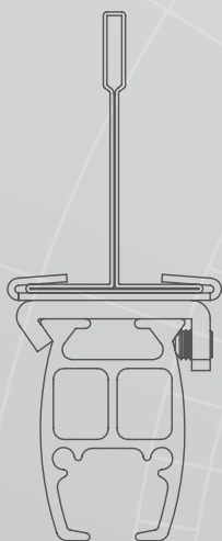
MTS Ceiling Bracket (for suspended ceiling)
