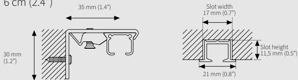
Milling dimensions KS Recess
