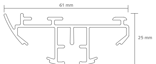
Motorised DS-XL Double LED Colours: white & matt black
