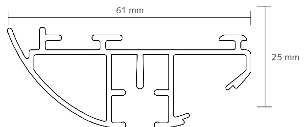
Motorised DS-XL LED Colours: white & anthracite
