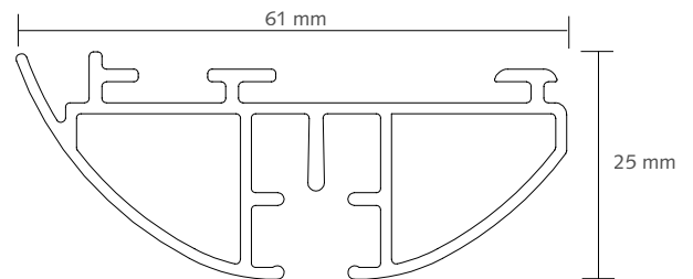
Motorised DS-XL Colours: matt white & matt black
